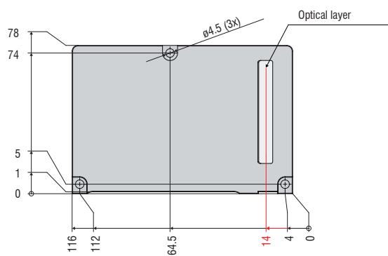
Receiver
