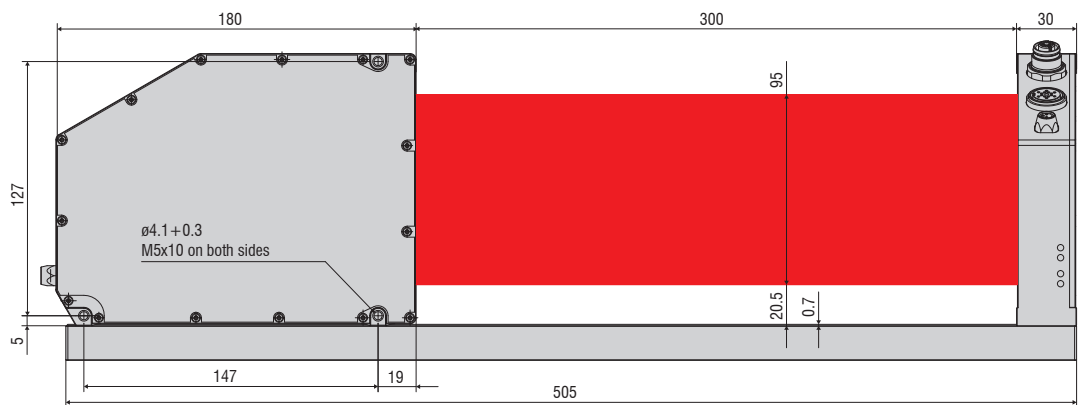
Light source
