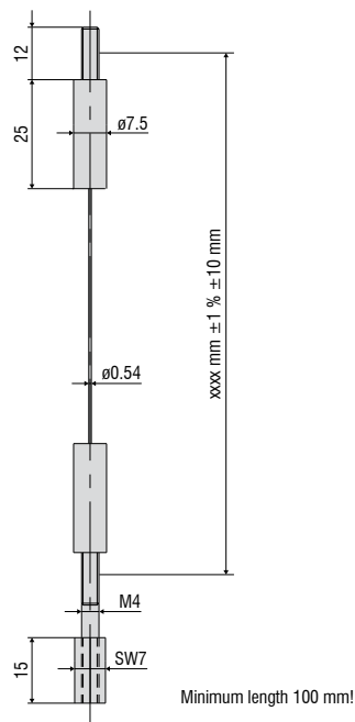
WE-xxxx-M4 Wire extension with M4 wire connection, x=wire length
