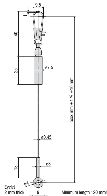
WE-xxxx-Clip Wire extension with eyelet, x = wire length
